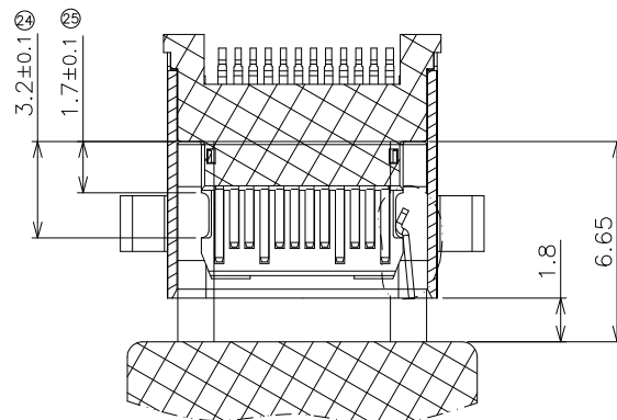
SECTION B-B MATTING VIEW
